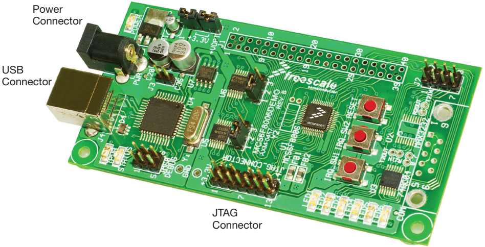
Figure 1. MC56F8006DEMO
